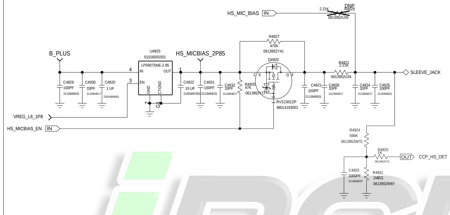
SENSOR HUB HEADSET DETECTION CIRCUIT
